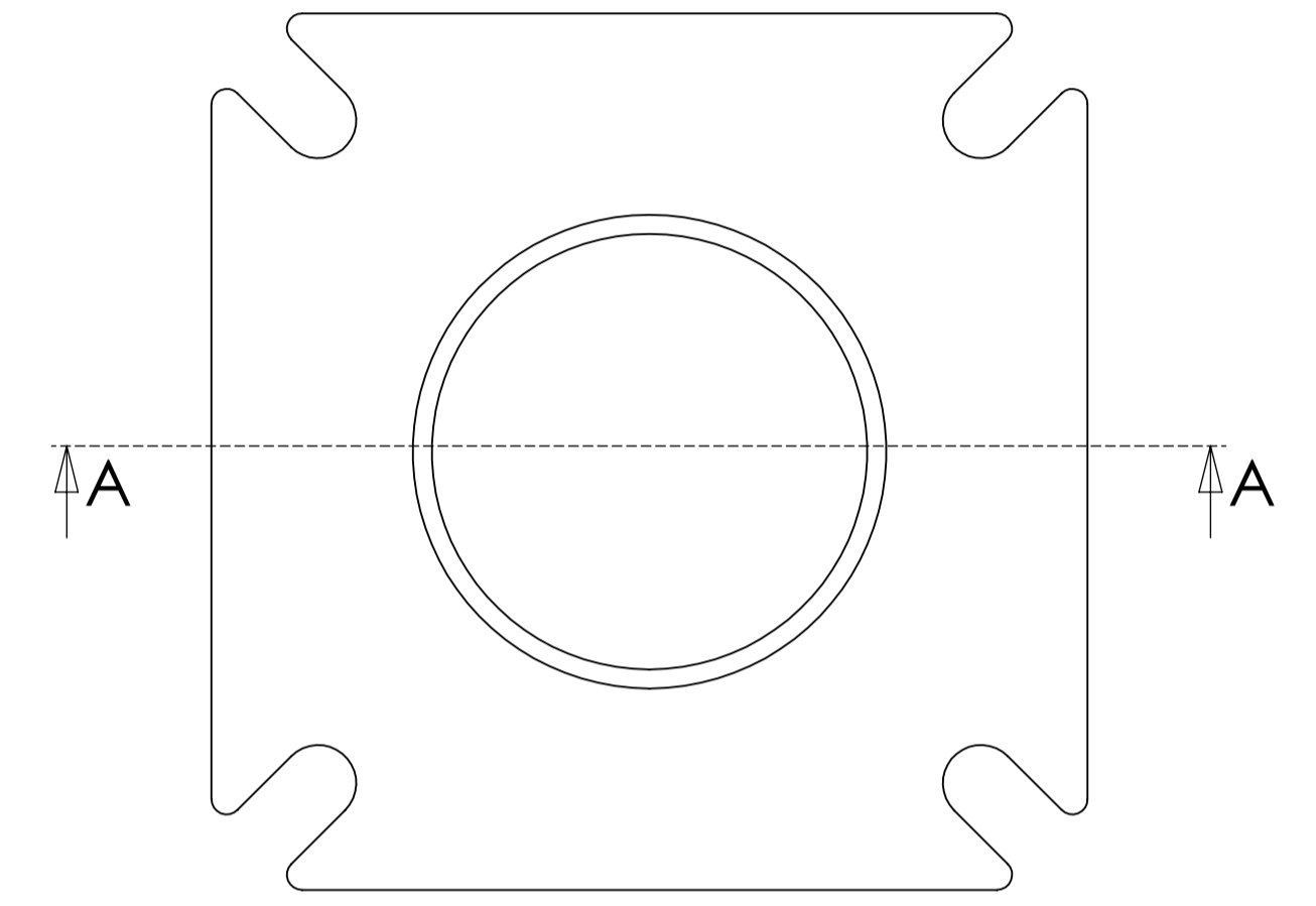
BASE PLATE WITH 4x FONDATION BOLTS
